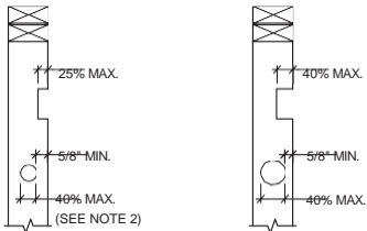
BEARING PARTITIONS & ALL EXTERIOR WALLS NON-BEARING PARTITIONS CRC FIG R602.6(1) & R602.6(2)
