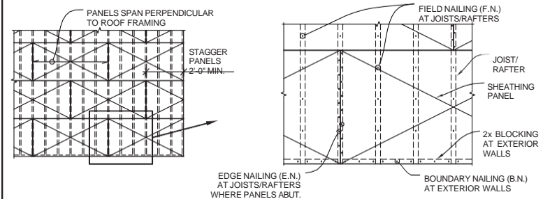
ROOF/FLOOR SHEATHING
