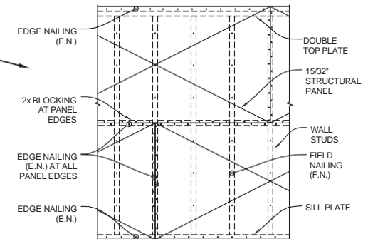
WALL SHEATHING
