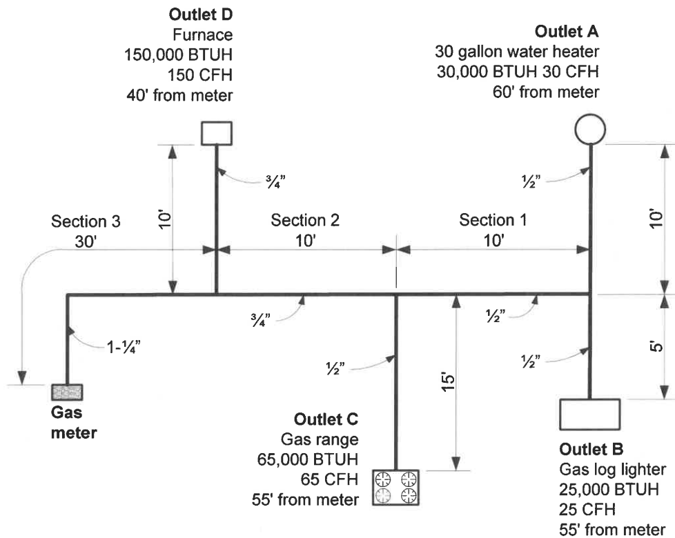
Figure C Example Piping Layout and Appliance Demand
